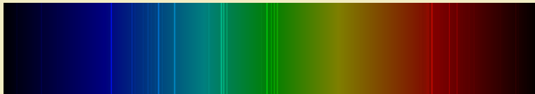
light spectral lines of the element strontium
