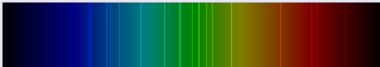
light spectral lines of the element radium
