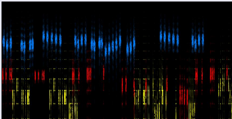
sound spectral germ-cell of radium colored in three layers
